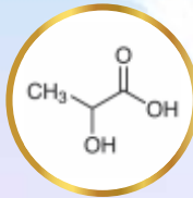
Lactic Acid
